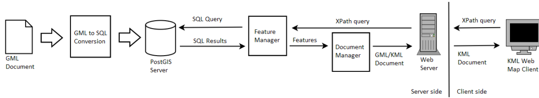
Figure 5: UALGIS System Architecture
