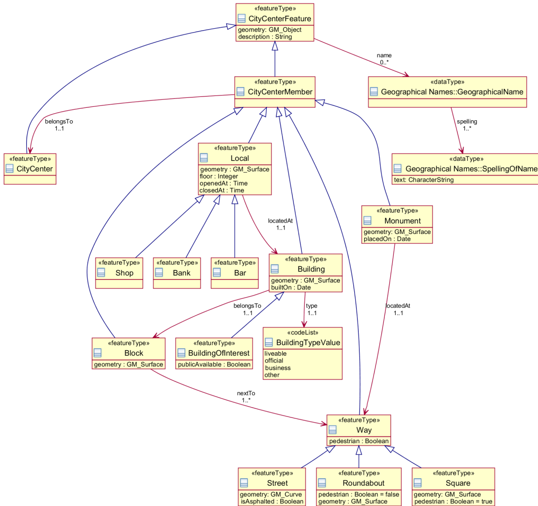
Figure 3: GML Schema of the City Center
