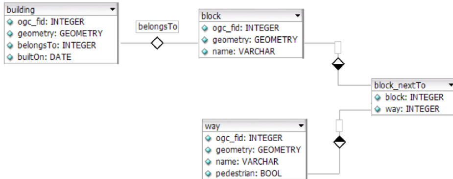
Figure 4: A Fragment of Relational schema of the City Center
