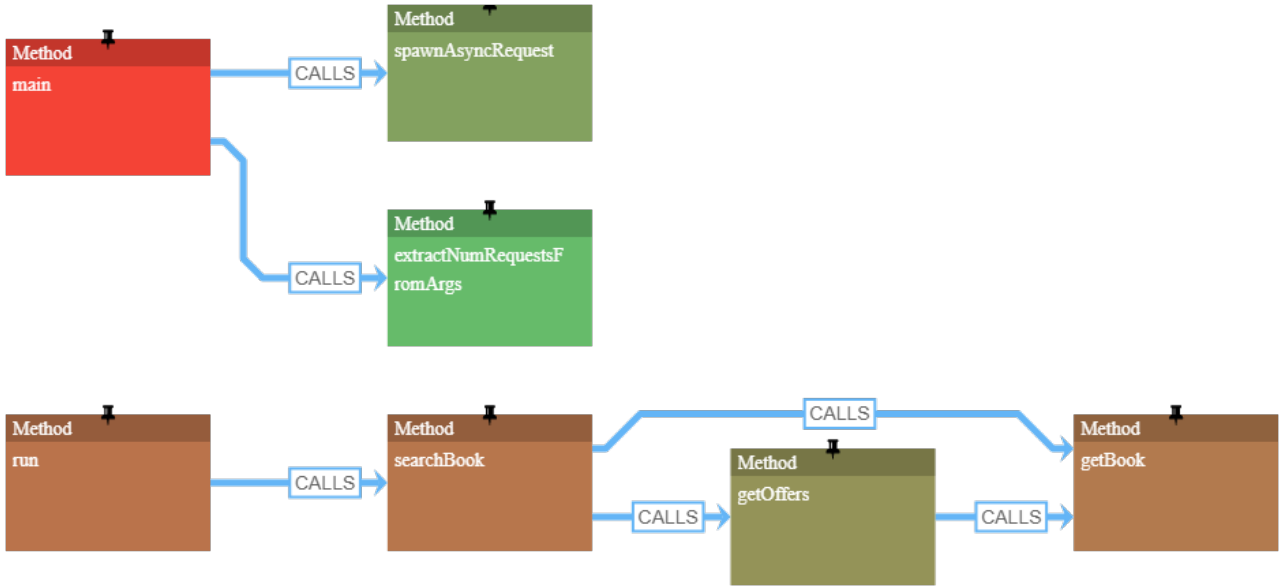
Figure 3: The call graph of the Bookstore application
