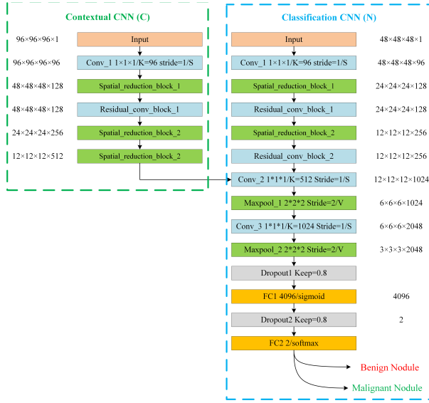
Figure 5. Architecture of contextual CNN for nodule classification.
