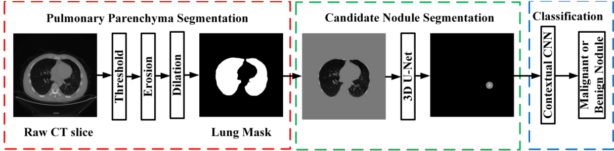
Figure 2. Overview of proposed lung nodule detection framework.
